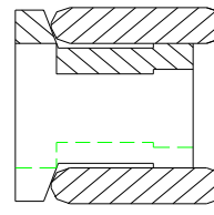
TPR - SOFT NITRIDED H' TYPE EXPANDER CODE : 308
