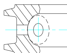
GNSOCH - GAS NITRIDED STEEL 2PIECE OIL RING CODE : 304
