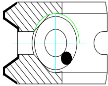
VZSOCH - OD CHROME CONFORMABLE OIL RING CODE : 302
