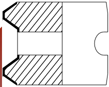
VZSOC - OD CHROME PLATED OIL RING CODE : 301
